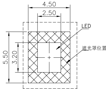
DETAIL C(4:1)
