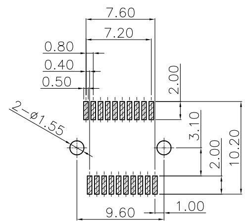
DETAIL A(SCALE 2:1)
