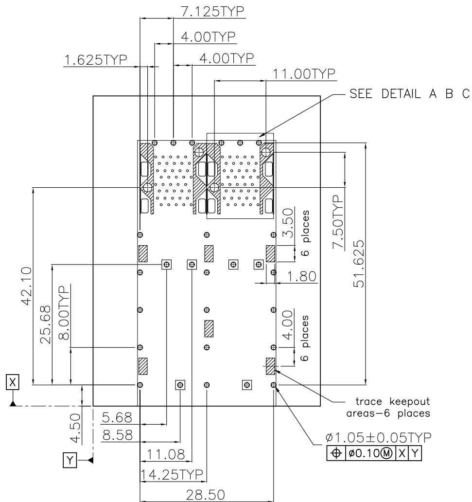
RECOMMENDED PCB LAYOUT (COMPONENT SIDE) PCB TOLERANCE \pm 0.05
