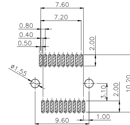
DETAIL A(SCALE 2:1)
