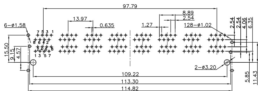
RECOMMENDED P.C.B LAYOUT TOP VIEW (COMPONENT SIDE TOLERANCE±0.05)
