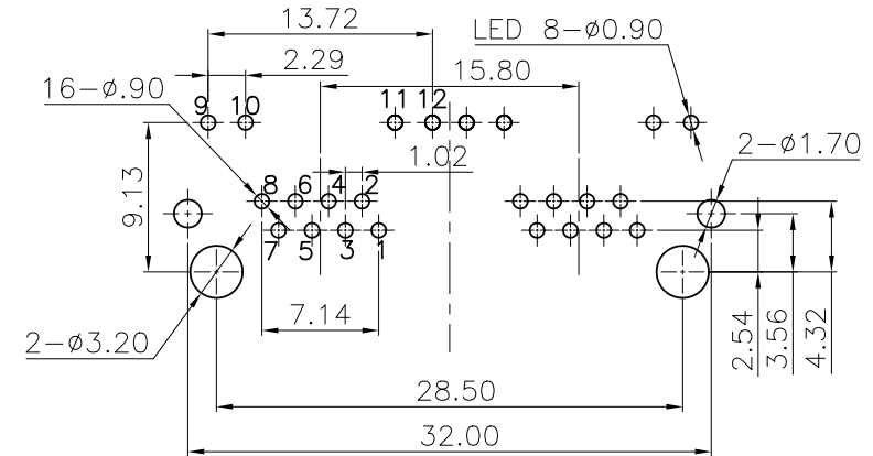
RECOMMENDED P.C.B LAYOUT TOP VIEW (COMPONENT SIDE TOLERANCE \pm 0.05 )
