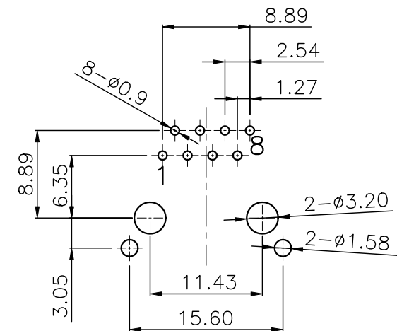
RECOMMENDED P.C.B LAYOUT(±0.05) TOP VIEW (COMPONENT SIDE)
