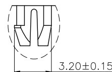
DETAIL A(2:1)
