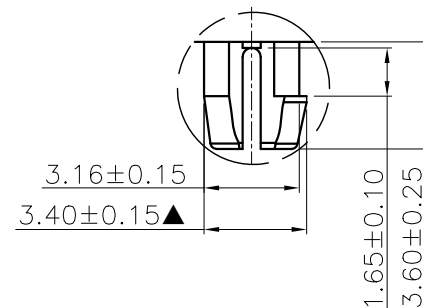
DETAIL A (2:1)
