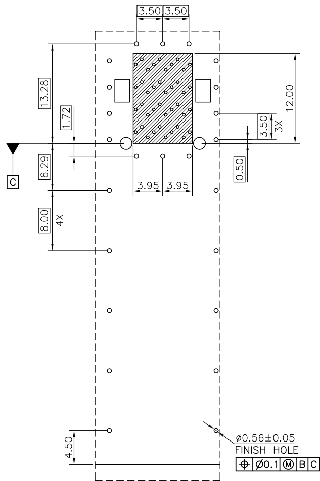
DETAIL A(2:1)
