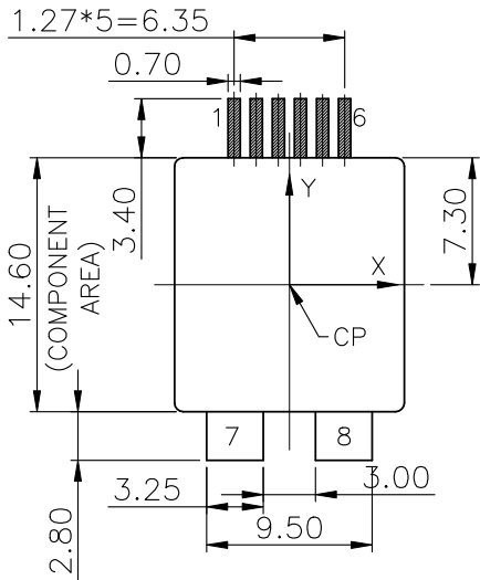
RECOMMENDED P. C. B LAYOUT TOP VIEW (COMPONENT SIDE TOLERANCE±0.05 THICKNESS=1.6mm)
